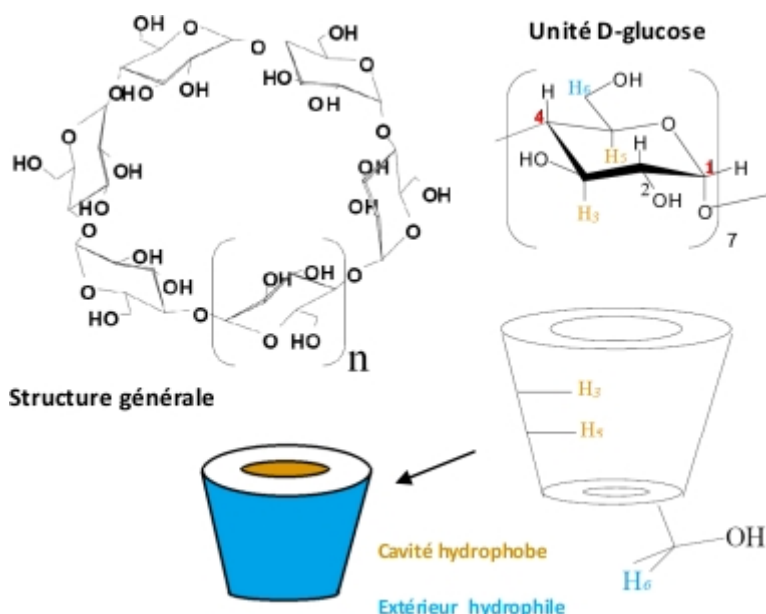
Figure 1. Structure des cyclodextrines.
